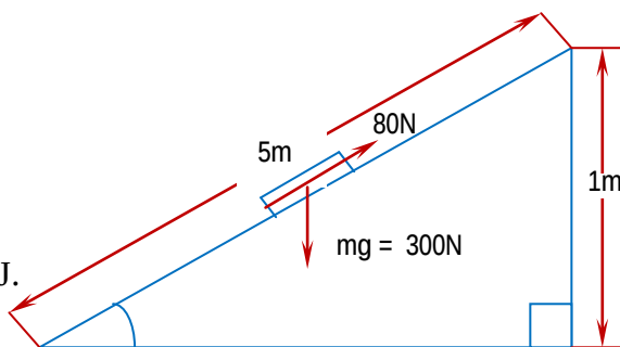
Fig 5.4 The efficiency of an inclined plane
