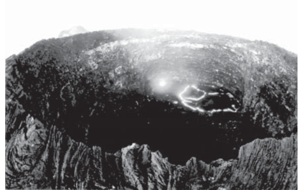
Ertale volcanic area
